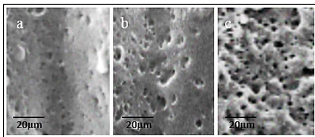
Figure 4. SEM images displaying the surface morphology of PMMA after KrF laser irradiation above the ablation threshold at a fluence of 800 mJ/cm 2 with different pulse numbers: a) 50, b) 100, and c) 150.
