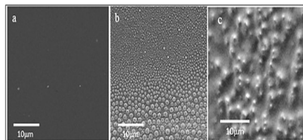
Figure 6. SEM images showing the surface morphology of PMMA after: a) CO 2 laser irradiation below the ablation threshold at a fluence of 500 mJ/cm 2 with 2000 pulses, b) CO 2 laser irradiation below the ablation threshold at a fluence of 500 mJ/cm 2 with 3500 pulses [1], and c) KrF laser irradiation below the ablation threshold at a fluence of 20 mJ/cm 2 with 10000 pulses.
