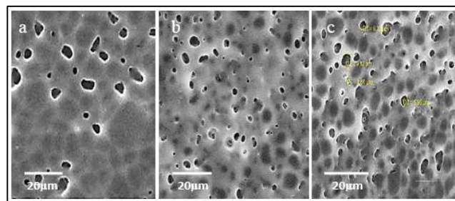
Figure 5. SEM images demonstrating the surface morphology of PMMA after CO 2 laser irradiation above the ablation threshold at a fluence of 2000 mJ/cm 2 with different pulse numbers: a) 50, b) 100, and c) 150 [1].
